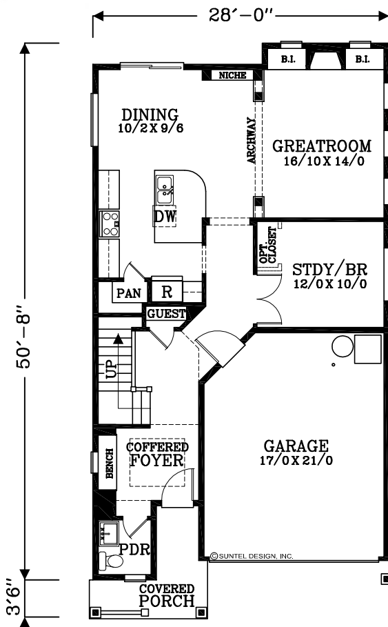
MAIN FLOOR PLAN 919 SQUARE FEET 2136 TOTAL SQUARE FEET
