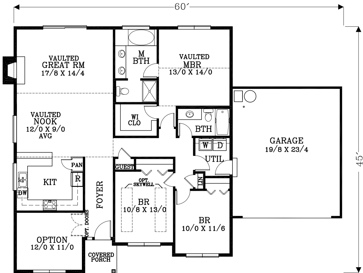
MAIN FLOOR PLAN 1670 TOTAL SQUARE FEET
