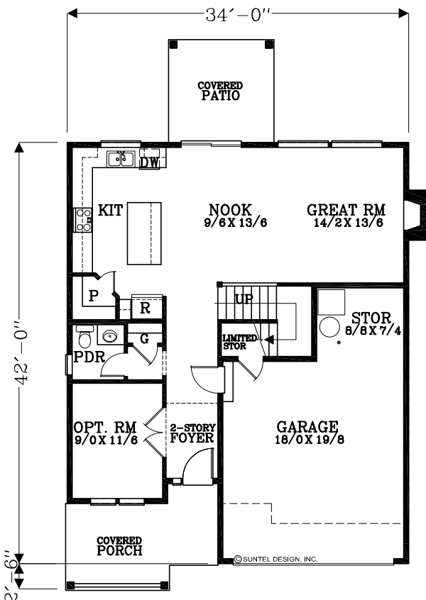
MAIN FLOOR PLAN 883 SQUARE FEET 2014 TOTAL SQUARE FEET
