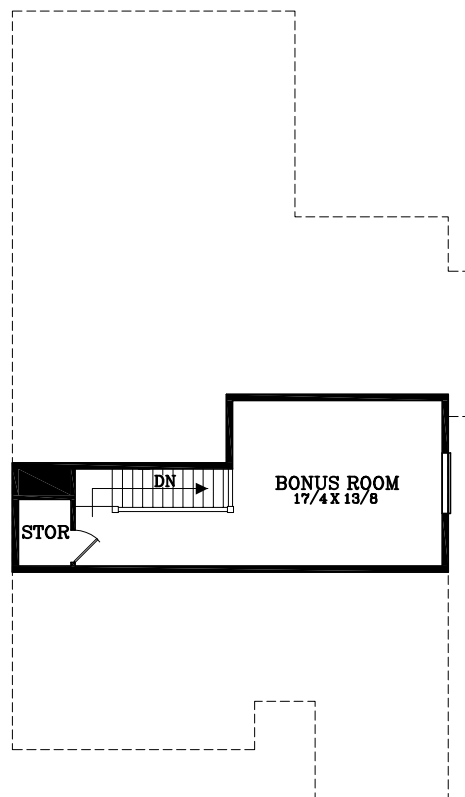
UPPER FLOOR PLAN 368 SQUARE FEET
