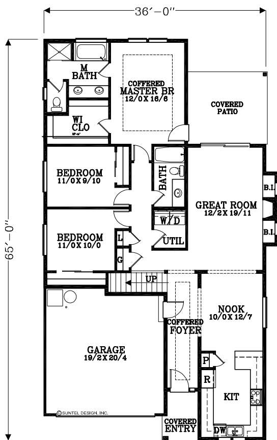
MAIN FLOOR PLAN 1634 SQUARE FEET 2002 TOTAL SQUARE FEET
