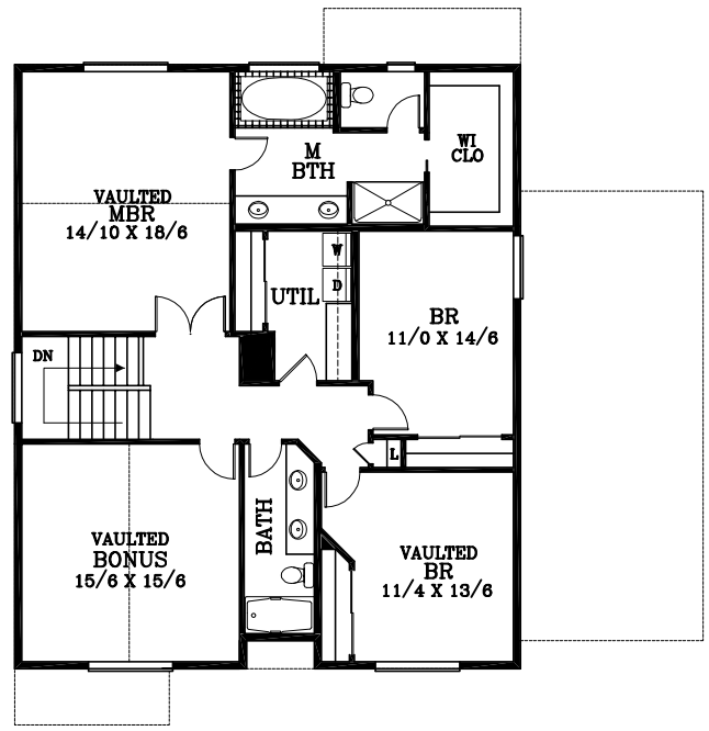
UPPER FLOOR PLAN 1466 SQUARE FEET
