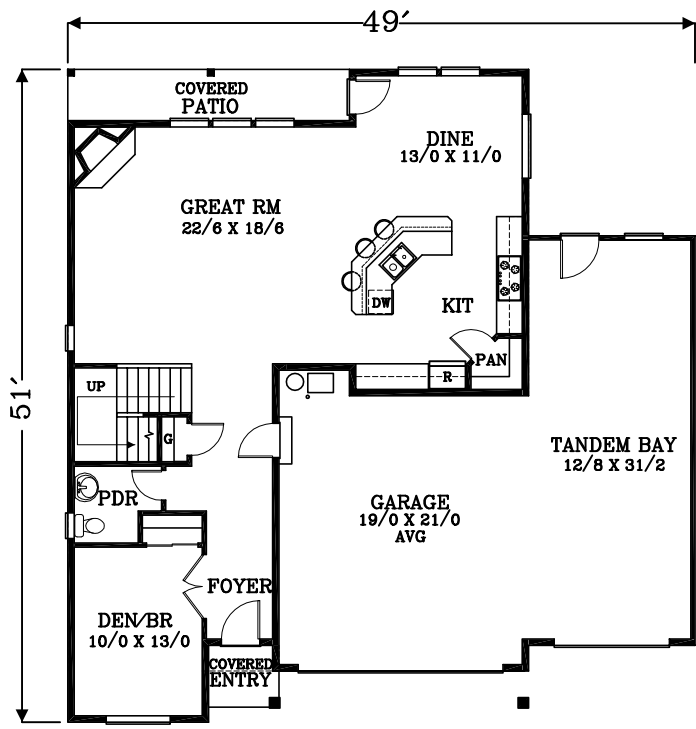
MAIN FLOOR PLAN 1213 SQUARE FEET 2679 TOTAL SQUARE FEET
