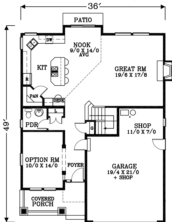
MAIN FLOOR PLAN 1086 SQUARE FEET 2417 TOTAL SQUARE FEET
