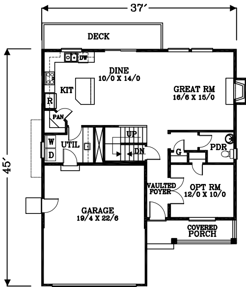
MAIN FLOOR PLAN 984 SQUARE FEET 3019 TOTAL SQUARE FEET
