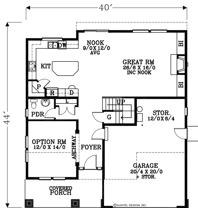
MAIN FLOOR PLAN 1082 SQUARE FEET 2377 TOTAL SQ FT
