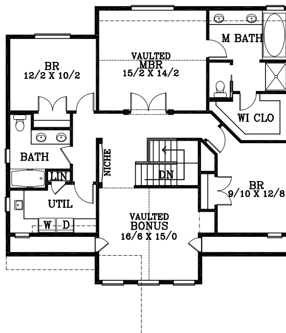
UPPER FLOOR PLAN 1295 SQUARE FEET INCL. BONUS ROOM
