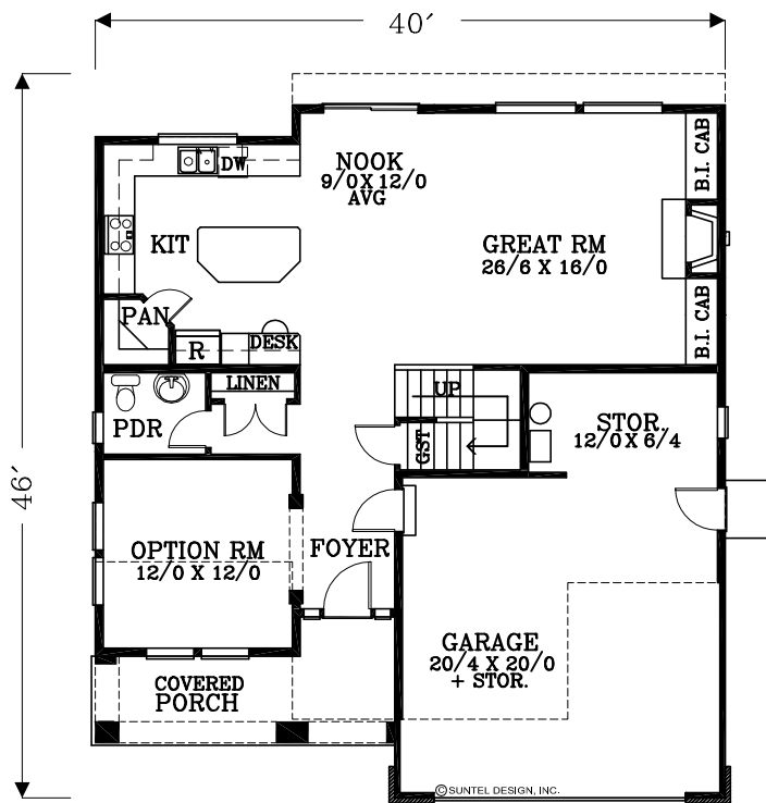
MAIN FLOOR PLAN 1020 SQUARE FEET 2335 SQUARE FEET TOTAL
