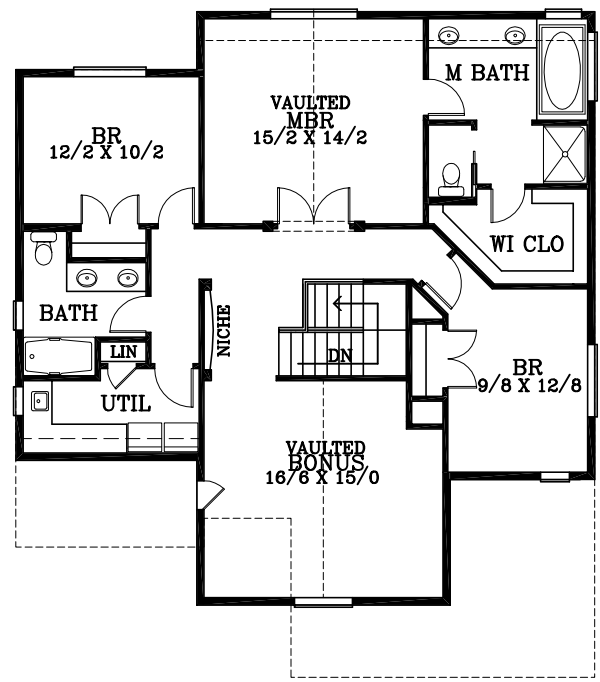
UPPER FLOOR PLAN 1315 SQUARE FEET
