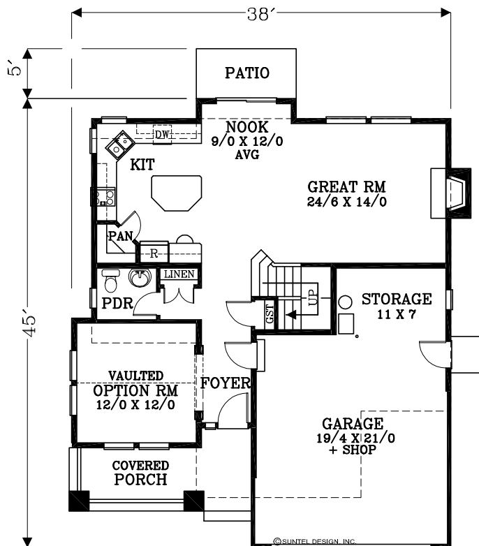
MAIN FLOOR PLAN 908 SQUARE FEET 1949 TOTAL SQUARE FEET
