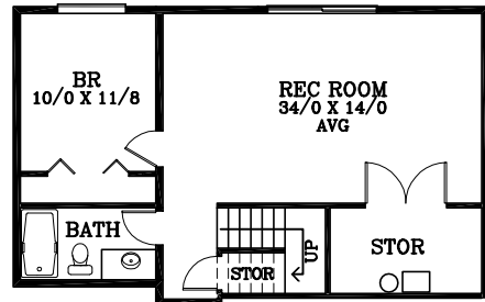
BASEMENT FLR PLN 748 SQ FT BONUS
