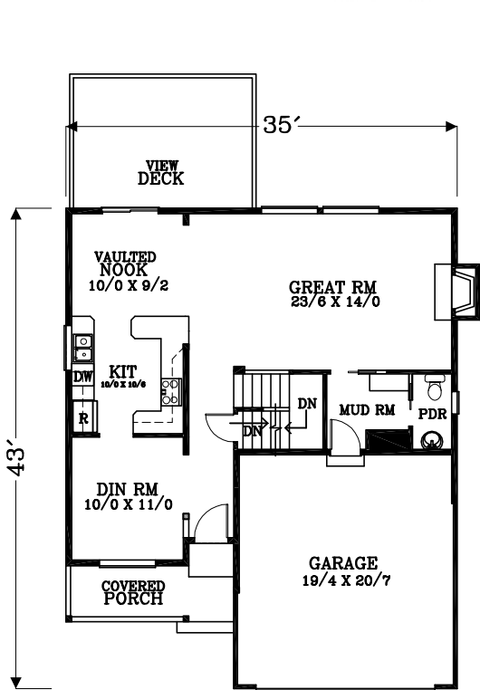
MAIN FLOOR PLAN 903 SQUARE FEET 2785 TOTAL SQ FT
