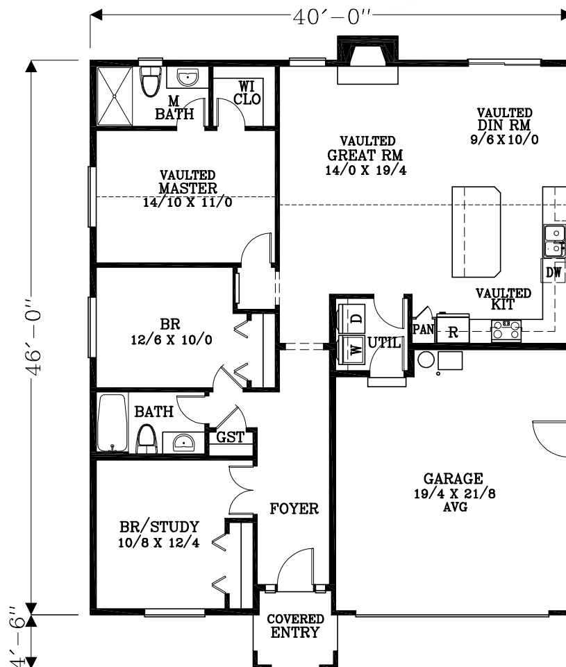
FLOOR PLAN 1389 SQUARE FEET
