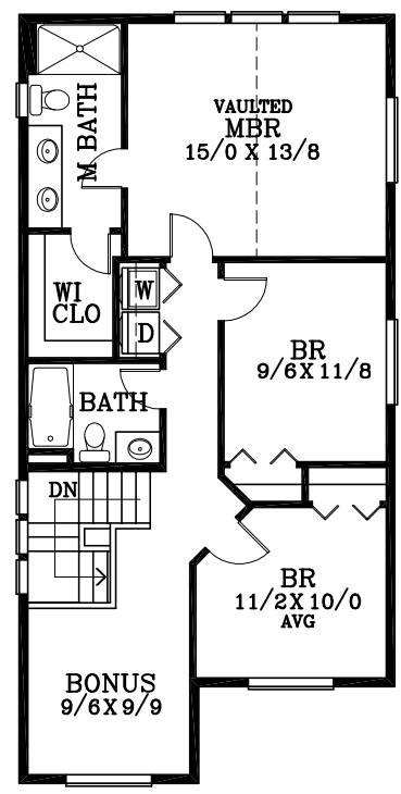
UPPER FLOOR PLAN 877 SQUARE FEET
