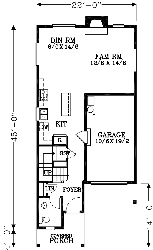
MAIN FLOOR PLAN 645 SQUARE FEET 1522 TOTAL SQUARE FEET
