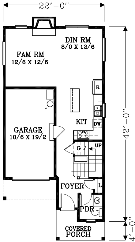
MAIN FLOOR PLAN 595 SQUARE FEET 1417 TOTAL SQUARE FEET
