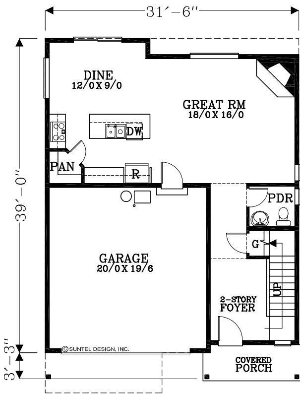
MAIN FLOOR PLAN 780 SQUARE FEET 1927 TOTAL SQUARE FEET
