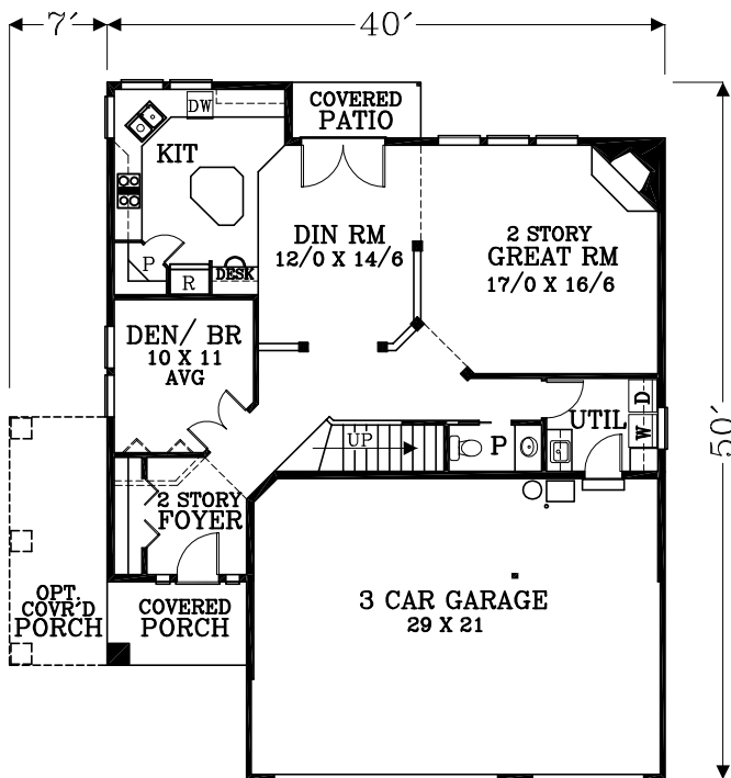
MAIN FLOOR PLAN 1104 SQUARE FEET 2146 SQUARE FEET TOTAL
