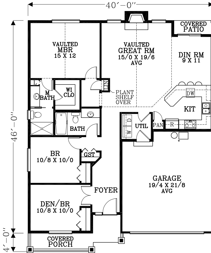
FLOOR PLAN 1371 SQUARE FEET
