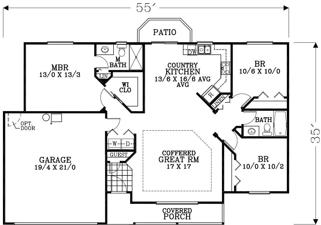
FLOOR PLAN 1263 SQUARE FEET
