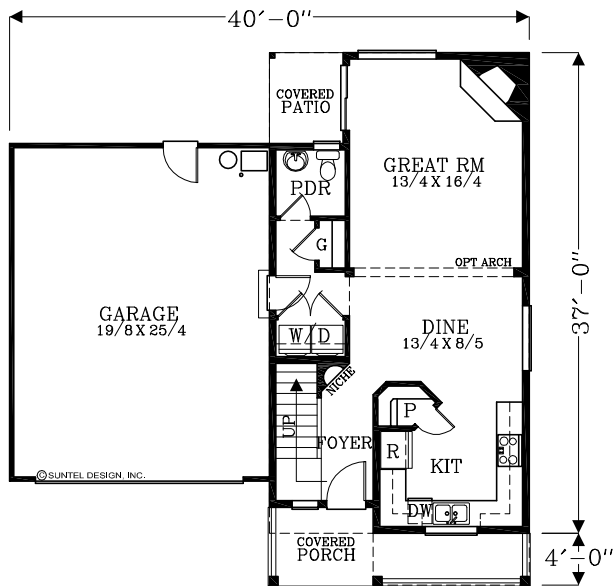
MAIN FLOOR PLAN 684 SQUARE FEET 1430 TOTAL SQUARE FEET
