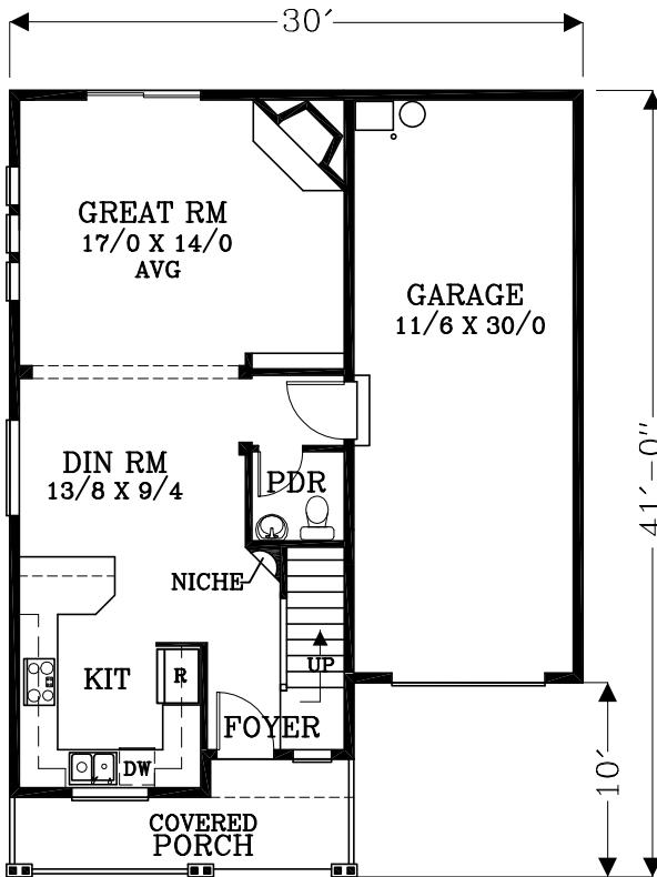
MAIN FLOOR PLAN 651 SQUARE FEET 1675 TOTAL SQUARE FEET
