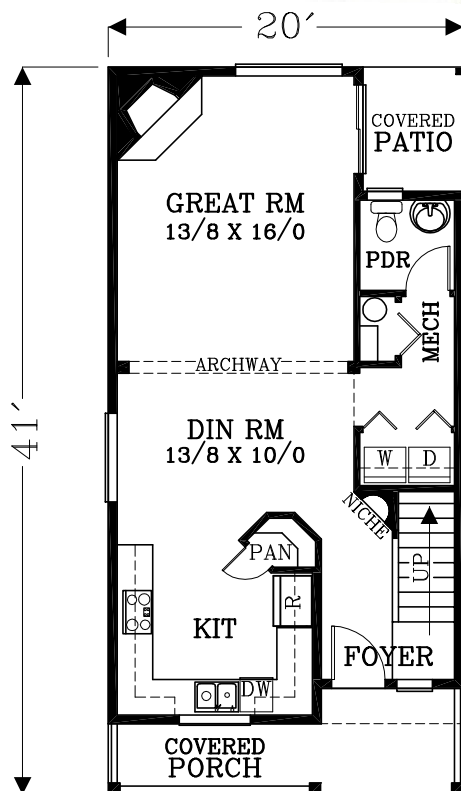
MAIN FLOOR PLAN 684 SQUIRE FEET 1428 TOTAL SQUARE FEET
