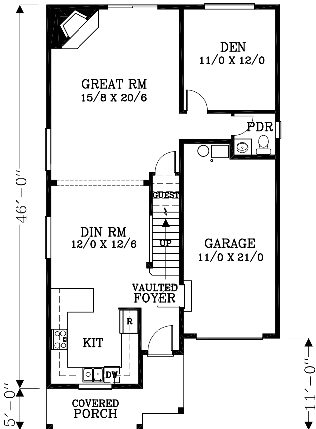
MAIN FLOOR PLAN 941 SQUARE FEET 1874 TOTAL SQUARE FEET
