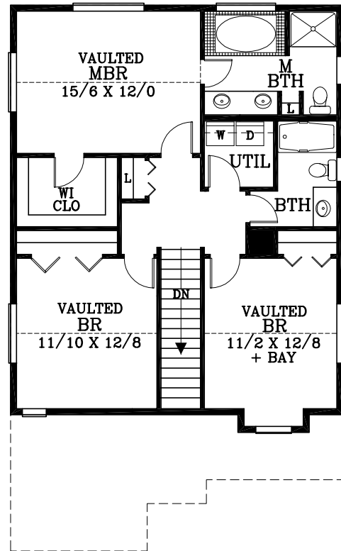
UPPER FLOOR PLAN 933 SQUARE FEET
