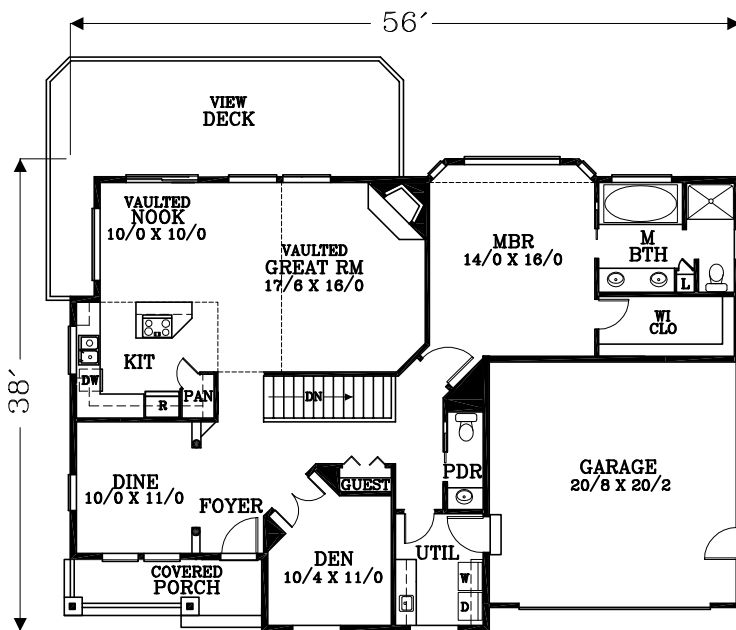
MAIN FLOOR PLAN 1545 SQUARE FEET 2389 TOTAL SQUARE FEET
