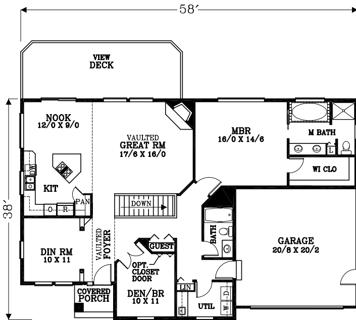
MAIN FLOOR PLAN 1635 SQUARE FEET 2638 TOTAL SQUARE FEET
