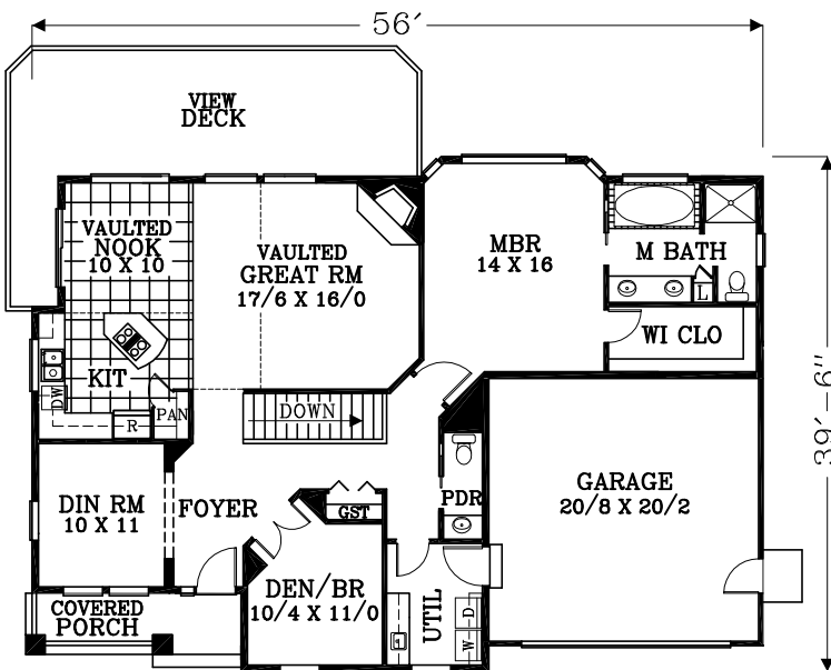
MAIN FLOOR PLAN 1545 SQUARE FEET 2389 S.F. TOTAL
