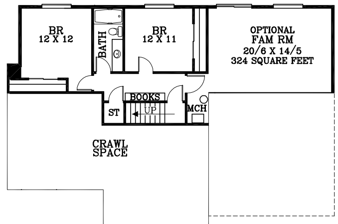
LOWER FLOOR PLAN 844 SQUARE FEET
