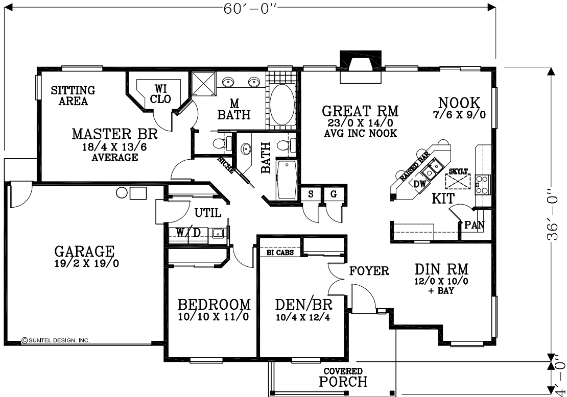
FLOOR PLAN 1615 TOTAL SQUARE FEET
