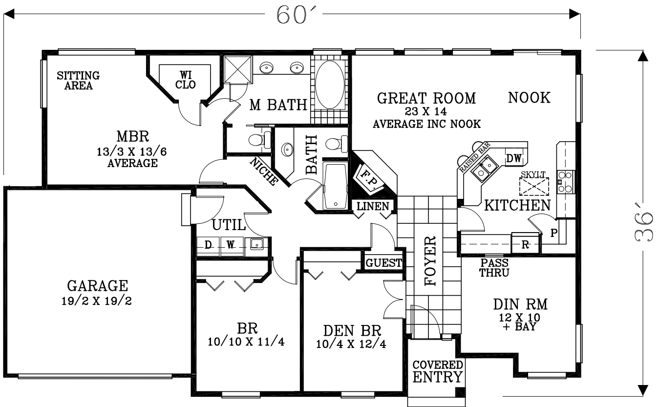
FLOOR PLAN 1607 SQUARE FEET
