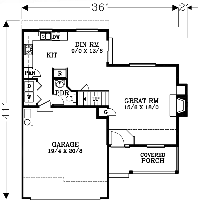
MAIN FLOOR PLAN 674 SQUARE FEET 1610 TOTAL SQ FT
