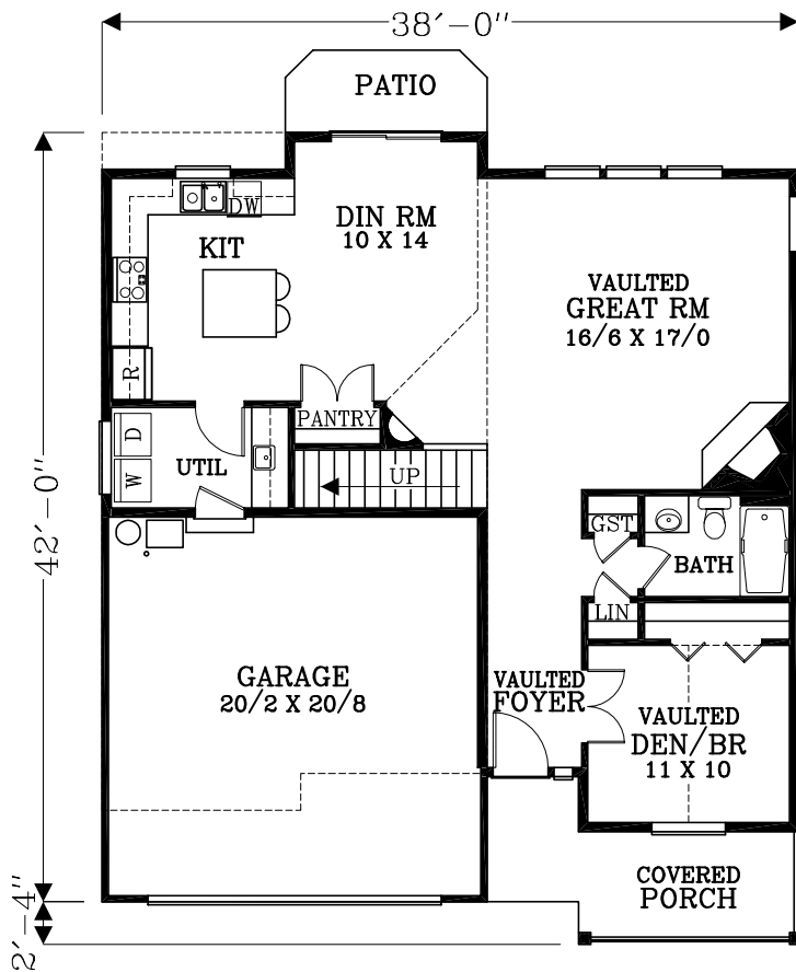
MAIN FLOOR PLAN 1027 SQUARE FEET 1749 TOTAL SQUARE FEET
