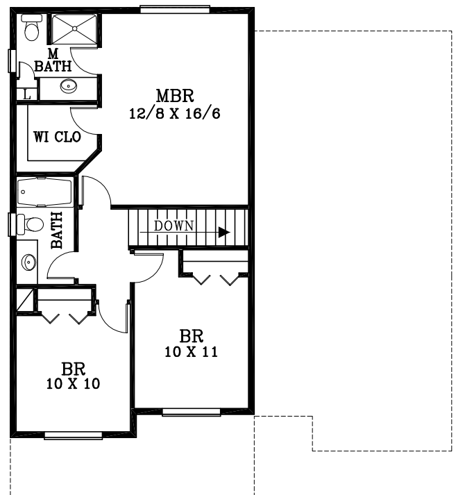
UPPER FLOOR PLAN 722 SQUARE FEET
