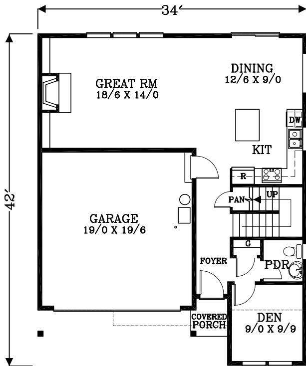
MAIN FLOOR PLAN 844 SQUARE FEET 2002 TOTAL SQUARE FEET
