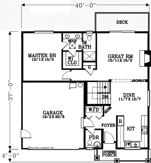
MAIN FLOOR PLAN 1050 SQUARE FEET 1765 TOTAL SQUARE FEET
