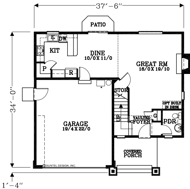
MAIN FLOOR PLAN 694 SQUARE FEET 1698 TOTAL SQUARE FEET
