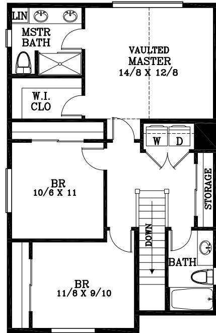
UPPER FLOOR PLAN 840 SQUARE FEET
