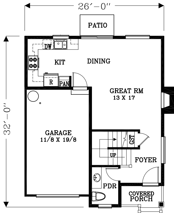
MAIN FLOOR PLAN 520 SQUARE FEET 1254 SQUARE FEET TOTAL
