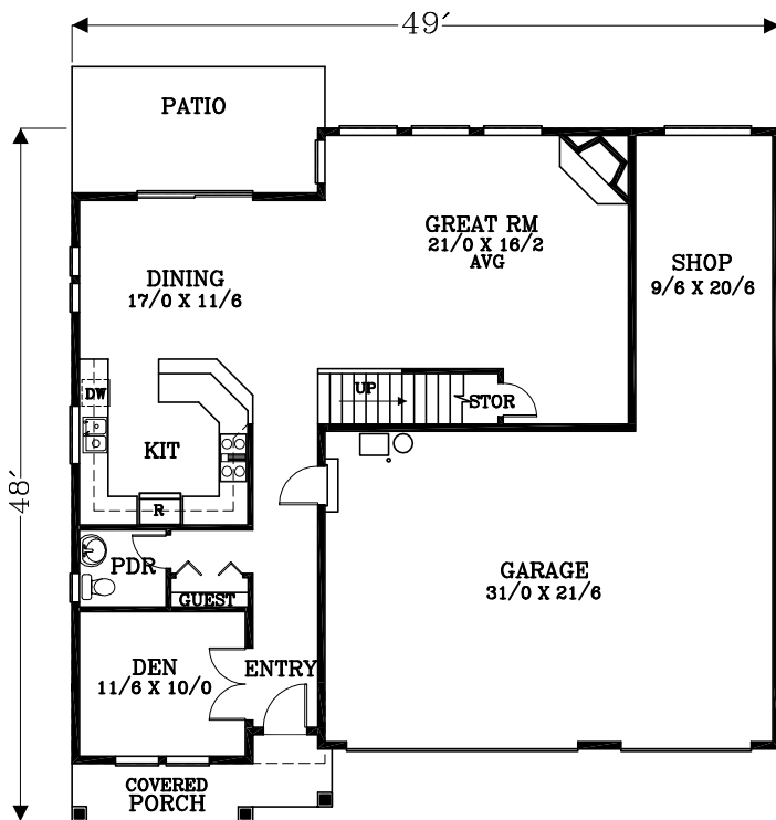
MAIN FLOOR PLAN 1135 SQUARE FEET 3066 TOTAL SQUARE FEET
