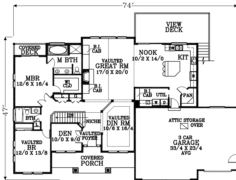
MAIN FLOOR PLAN 1944 SQUARE FEET 3014 TOTAL SQUARE FEET
