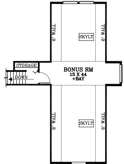
UPPER FLOOR PLAN 775 SQUARE FEET
