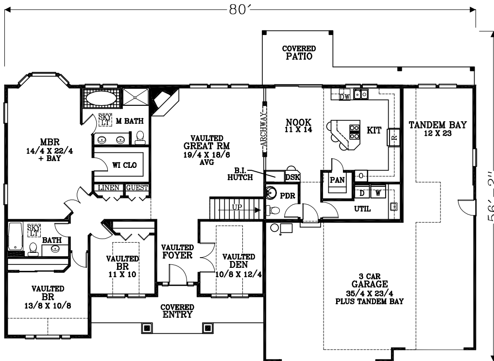
MAIN FLOOR PLAN 2243 SQUARE FEET 3018 TOTAL SQUARE FEET
