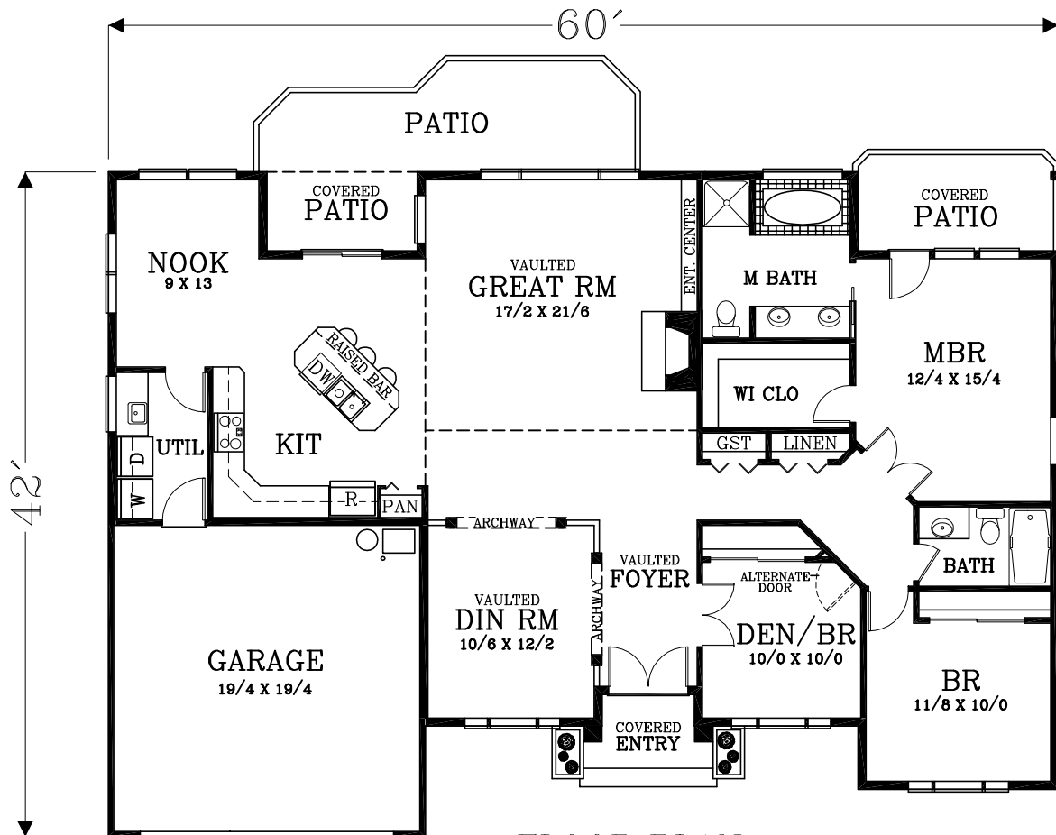
FLOOR PLAN 1779 TOTAL SQUARE FEET
