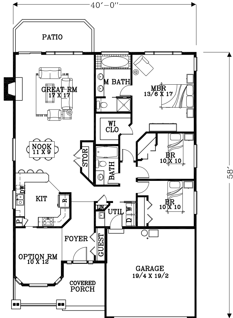
FLOOR PLAN 1732 SQUARE FEET
