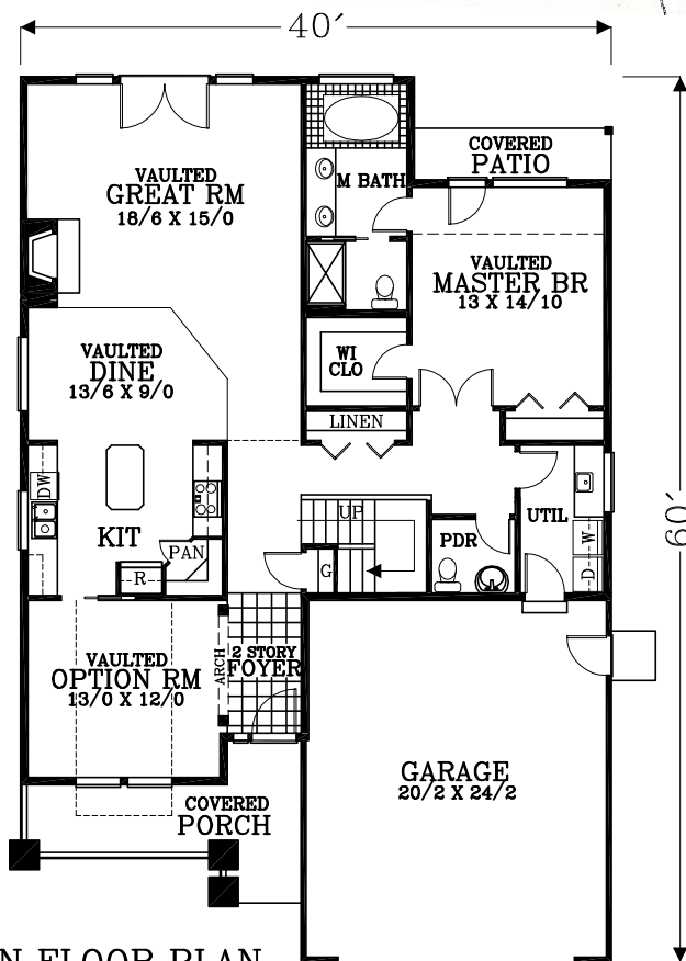
MAIN FLOOR PLAN 1501 SQUARE FEET 2044 SQ FT TOTAL
