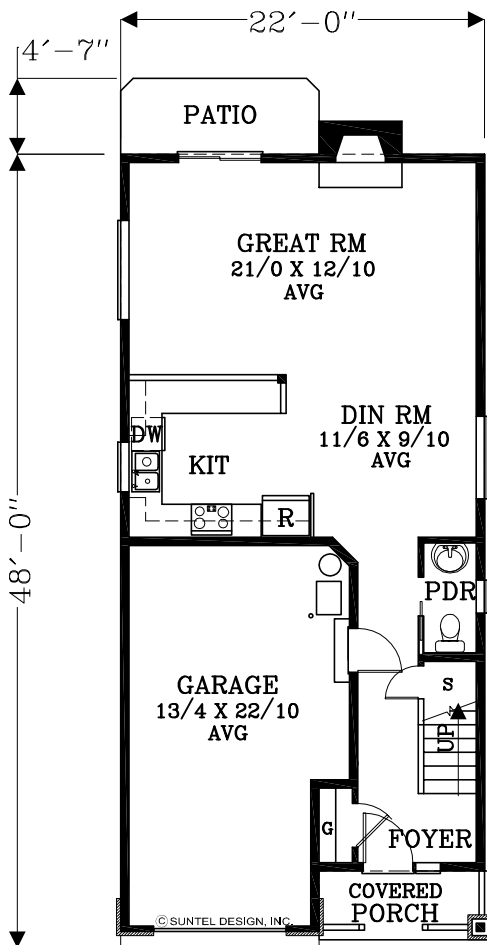
MAIN FLOOR PLAN 695 SQUARE FEET 1668 TOTAL SQUARE FEET
