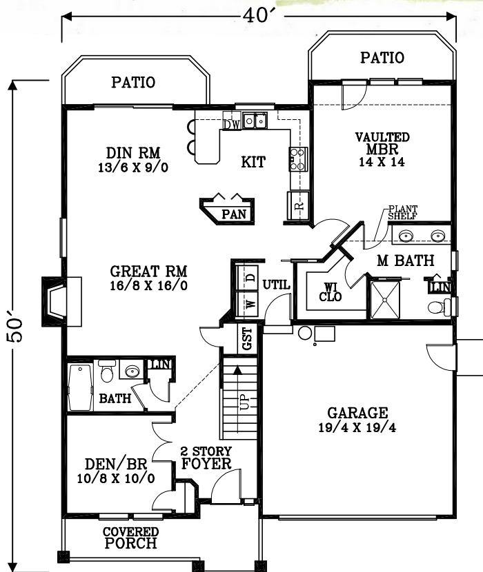
MAIN FLOOR PLAN 1300 SQUARE FEET 1748 TOTAL SQUARE FEET
