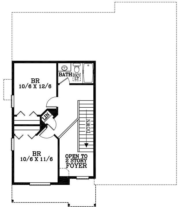
UPPER FLOOR PLAN 448 SQUARE FEET
