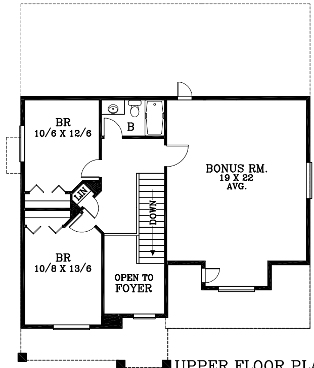
UPPER FLOOR PLAN 1051 SQUARE FEET
